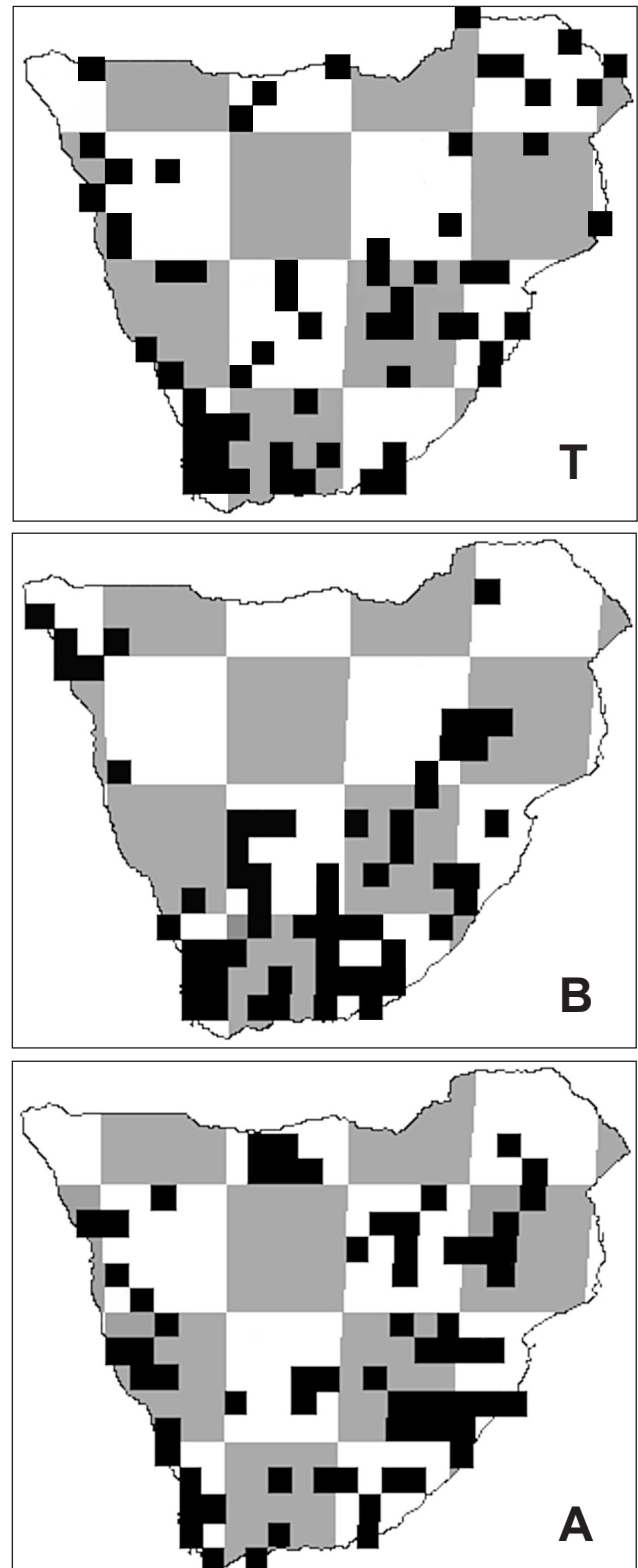
Figure 2: Distribution of type localities (T), Barn Owl roosts (B) and archaeological (A) sites in southern Africa. Black squares represent degree squares from which specimens have been collected. White and grey squares are five degrees on a side. See Appendix 3 for additional information.
